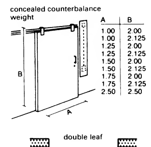
14 Sliding fire doors T30-T90
